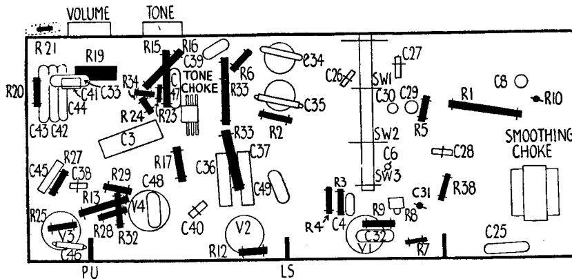
Above, is the diagram showing how parts are situated underneath the chassis of the 785 AX. The "top deck" view is given on the right. C14 and C15 are between the band-pass coils and the gang.
