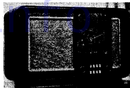
The Philips 660A is a 4-valve plus rectifier three-band superhet with a unique form of push-button mechanical tuning. The buttons operate a special "linear action" gang condenser and neither pre-set circuits or motor are required.
