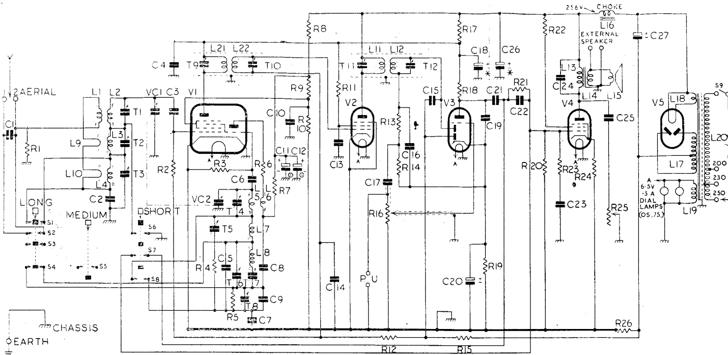
WAVE CHANGE SWITCH SHOWN WITH M.W. BUTTON IN OPERATED POSITION. SWITCH S9 IS CLOSED WHEN A WAVE RANGE BUTTON IS OPERATED. * CONDENSERS C18, C19, C20, C21 HAVE A COMMON NEGATIVE FOIL. © C11, C12
