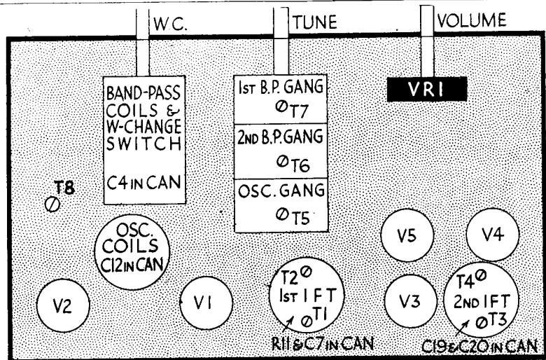
These two diagrams of the Ekco chassis, in conjunction with the tables on the left, enable all the component parts to be identified. Above is the top-of-chassis diagram.
