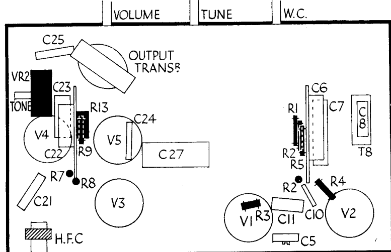
Even underneath the B67 chassis is quite clean and simple. Most of the small parts are suspended in the wiring and thus occupy their "logical" positions.
