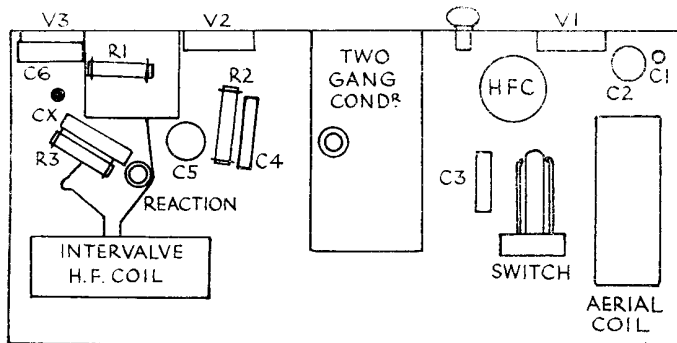
Only the valves are mounted on the top of the chassis of the Burgoyne receivers, and so only this under-chassis layout need be given.
