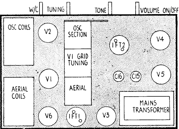
Left is the layout of the upperside of the chassis of the Belmont Model 700 all-wave superhet.
