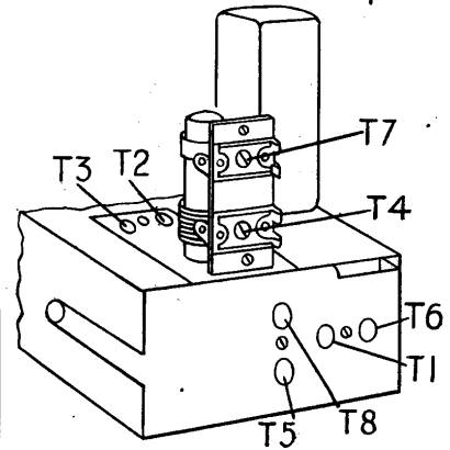
Three bands are covered by this compact receiver and the trimmers are located as shown in this diagram.
