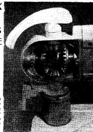
Fig. 6—Wriinger is fitted with a Swirlux gearbox seen here with outer casing and one coverplate removed
