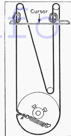
Right: Sketch showing the tuning drive system, as seen from the front with the gang at maximum.
