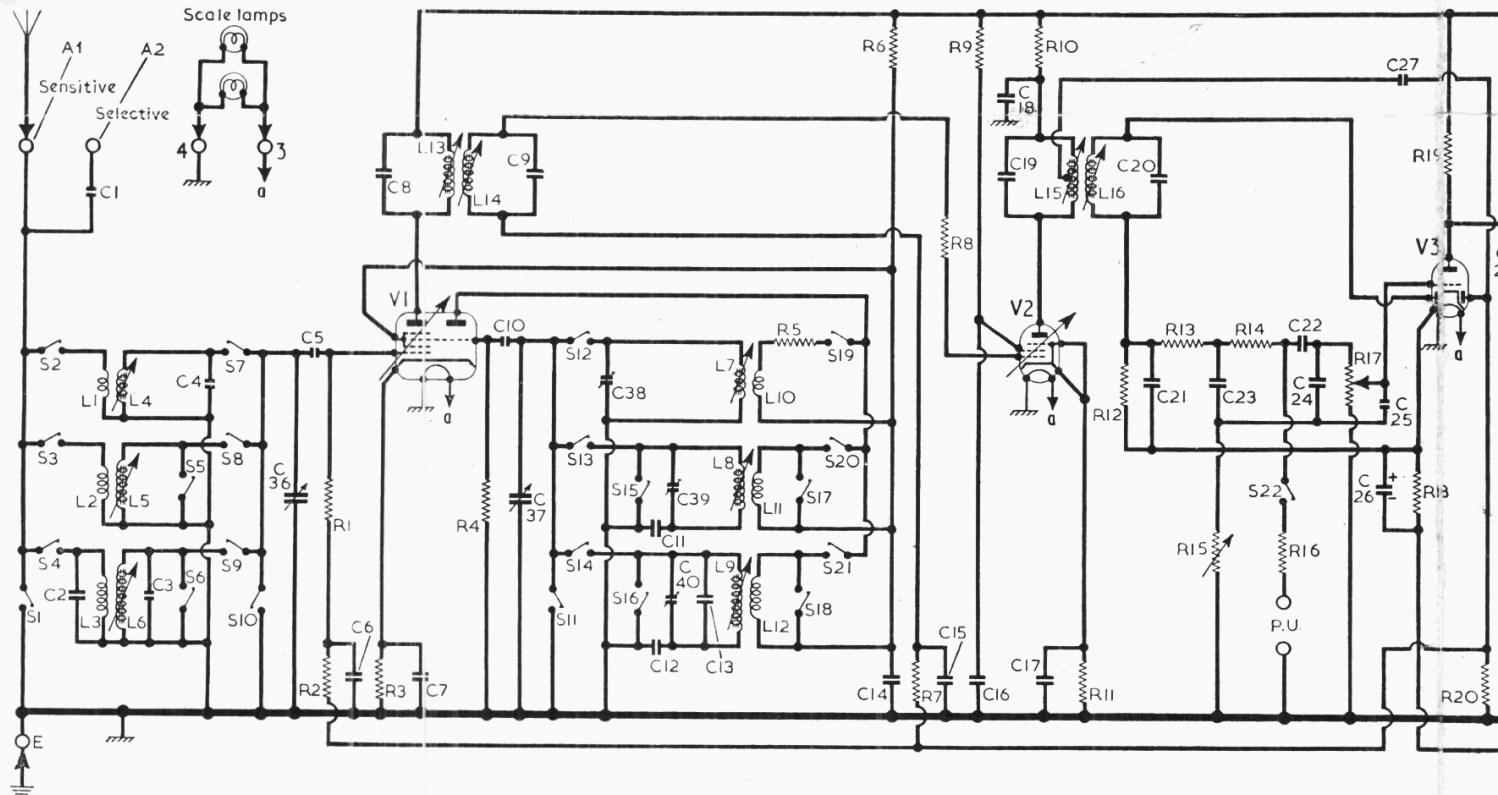
Circuit diagram of the Bush SUG 26 superhet. The variable tone control circuit is unusual, and consists of C23, R14, C24 and R15 in the circuit. Fixed negative feed-back is applied from the speech coil circuit to the cathode of V3 , and it is modified on gram by the closing of switch S22 . The numbered interconnecting points around the scale lamps and output transformer circuit represent the pins of an octal-type connector between certain components mounted in the cabinet.
