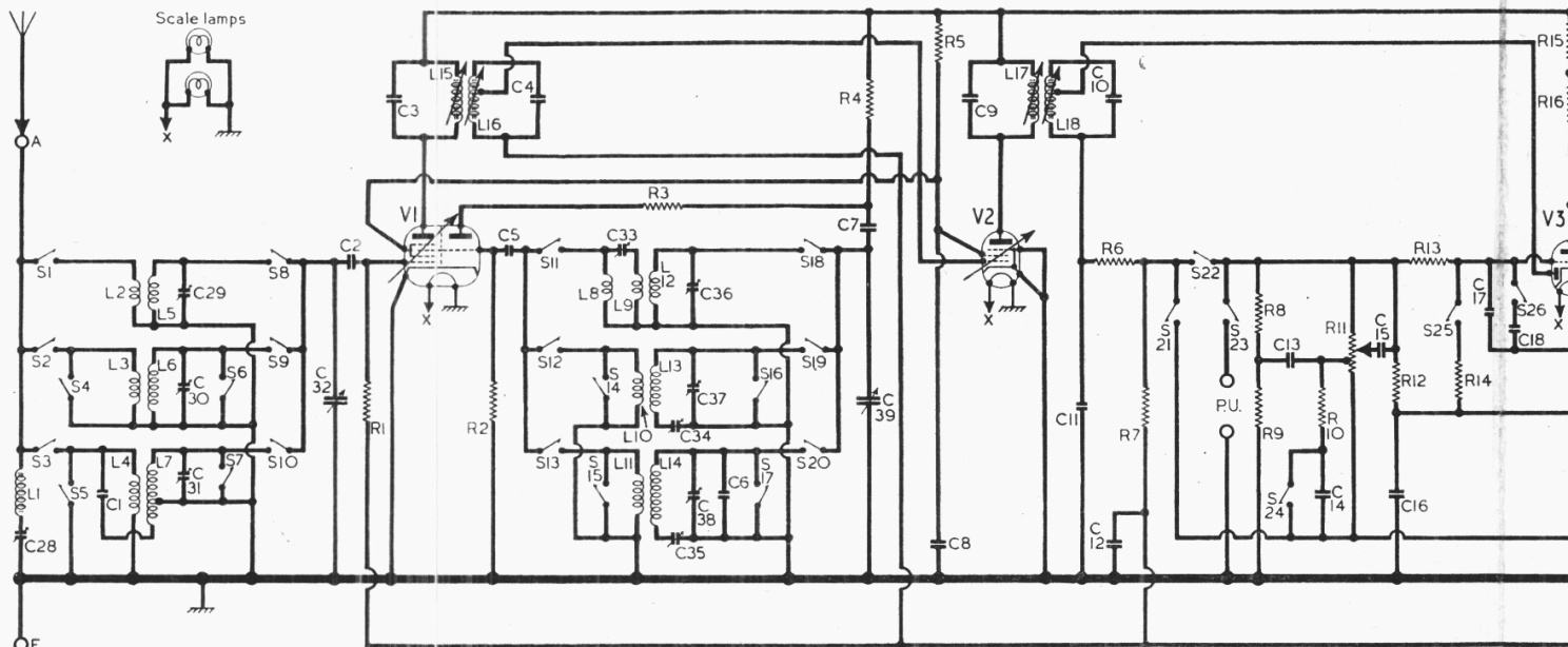
Circuit diagram of the Philips 400A and, with the addition of a cat tuning indicator, the 500A. The circuit diagram of the C.R. indicator at the foot of col. 6. Four degrees of feedback, derived from the speaker circuit, are applied at various points in the audio frequency circuit, with which is the 5-position tone control device. Special measures have been adopted in the L.W. aerial coupling circuit to maintain a constant efficiency throughout the band.
