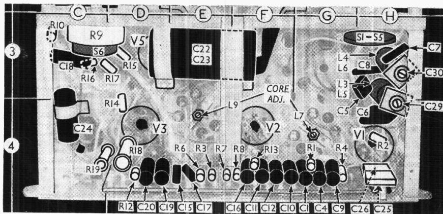
Under-chassis view. A detailed diagram of the waveband switch unit S1-S5 is inset in the top left-hand corner of the circuit diagram overleaf.
