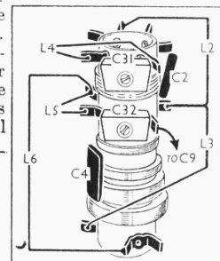
Sketch identifying the aerial coil unit tags.
