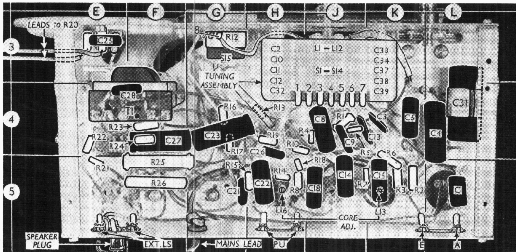
Under-chassis view. The position of the tuning assembly is indicated here, and the numbers of the components it contains are listed. The seven tags are numbered to agree with the same connections in the circuit diagram overleaf. An eighth connection consists of a systoflex covered lead which goes to the volume control.
