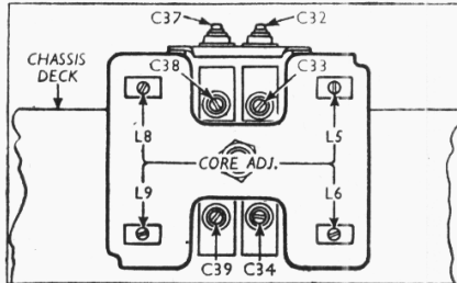
Sketch showing the front of the tuning assembly, on which are mounted all the R.F. and oscillator trimmers and core adjustments. Reference is made to this sketch in "Circuit Alignment."
