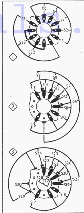
Diagrams of the three waveband switch units, drawn as seen when viewed from the rear of an inverted chassis, the top diaphragm here being the front unit in the chassis. The associated switch table is on the right.
