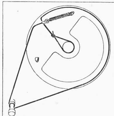
The course taken by the drive cord, as it would be seen from the rear.
