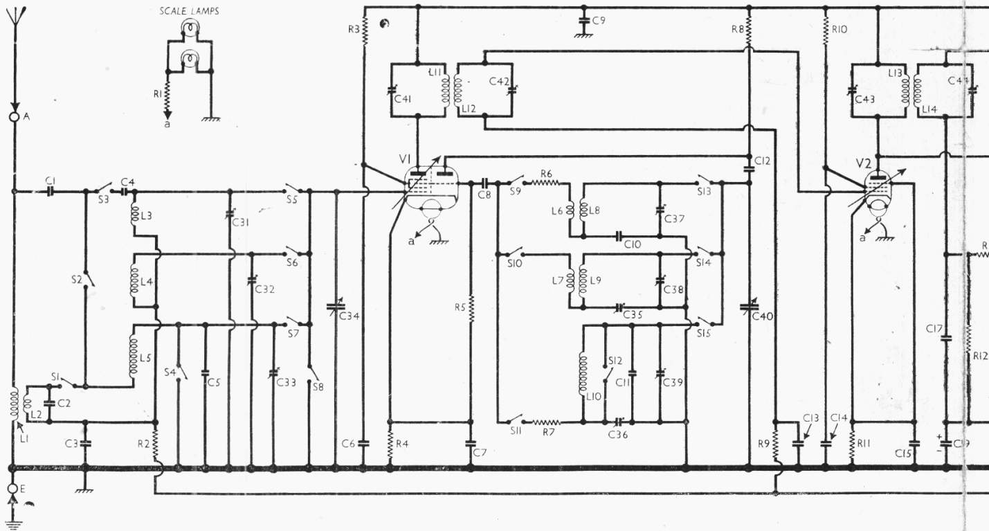
Circuit diagram of the Ferguson 461 3-band A.C. superhet. On L.W., the aerial tuning coil L5 is bottom-coupled by the line forms the secondary winding of the aerial transformer L1 , L2 , switch S1 then being closed. On M.W., S1 opens and S2 , "inverting" L5 and connecting it between aerial and earth. L5 then operates as the M.W. aerial coupling coil. R19 , C24 in V1 provide negative feed-back voltages whose character is varied by adjusting the tone control R19 . These are coupled back to V2 via R17 . In early chassis C22 , R16 and R17 were omitted, and R19 was then returned to chassis.
