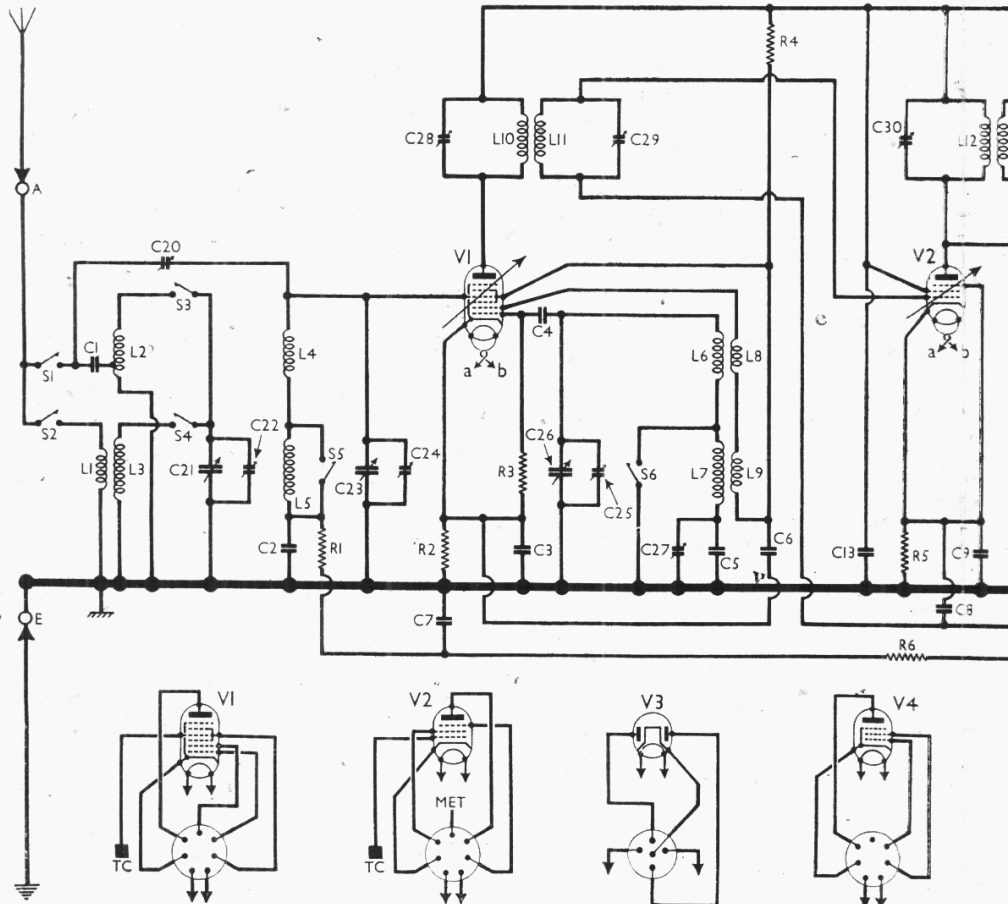
Circuit diagram of the Ekco AC77 AC superhet and the console model CT77. The separate power pack is connected to the chassis by connections numbered 1 to 10. These numbers are repeated in our illustration of the unit of the mains transformer section of the mains transformer.
