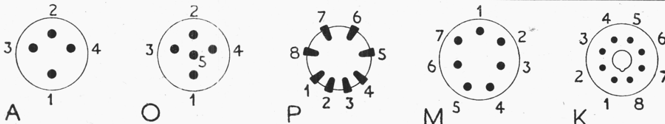
Diagrams of the five bases concerned, viewed from the free ends of the pins, showing the pin numbers as they appear under "Remarks."
