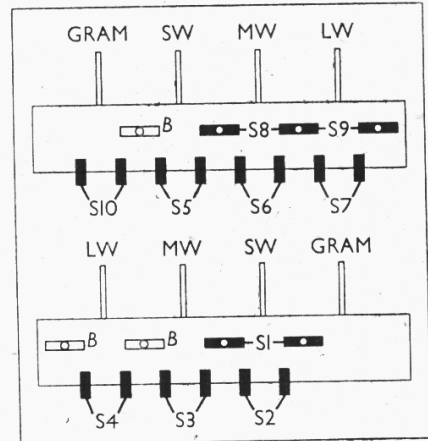
Diagrams of both sides of the switch unit. The upper one shows the switches seen from the underside of the chassis, while the lower one shows those on the side facing the chassis deck.
