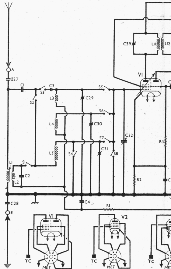
Circuit diagram of the Ferguson 101U AC/DC superheterodyne receiver.
