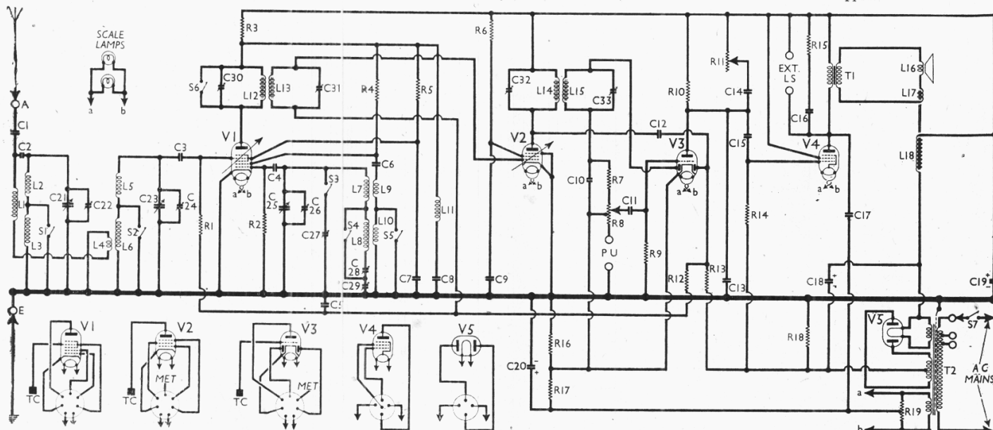
Circuit diagram of the Coszor 375 AC superhet. An identical chassis is employed in the model 385. R8 is the fader type volume control.
