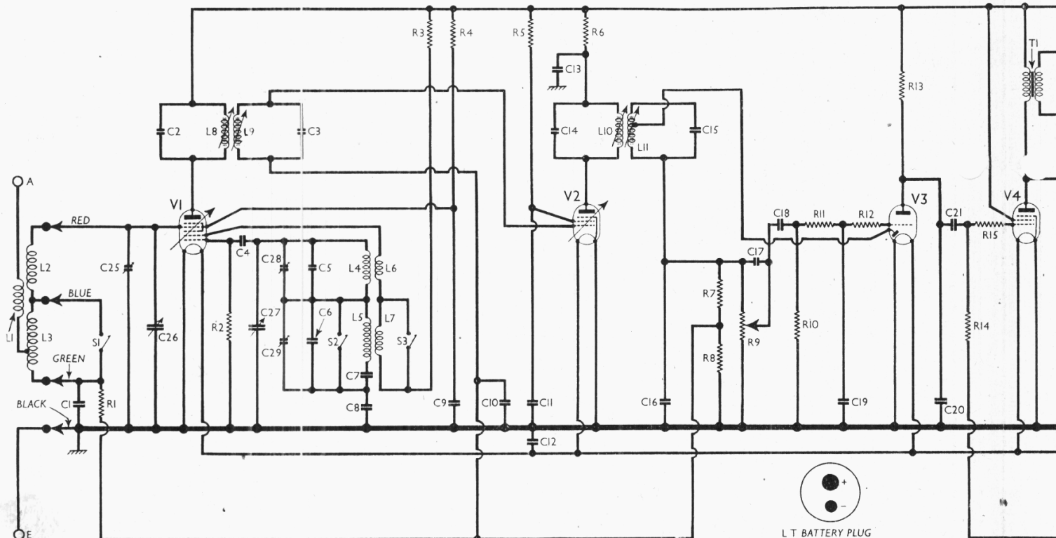
Circuit diagram of the Philips 229B portable all-dry superhet. An accumulator may be used if desired, as explained in "General Notes." For earth connections via the coupling winding L1 . The frame aerial connections are indicated in the diagram. Diagrams of the base connections are on the right of the circuit diagram.
