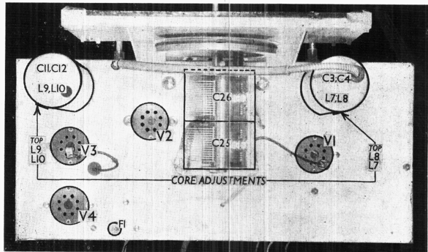
Plan view of the chassis. The IF core adjustments are indicated. Each IF transformer also contains its fixed trimming capacities.
