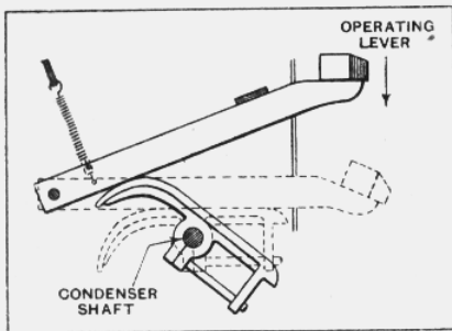
Fig. 3.—Control bar operated unit.
