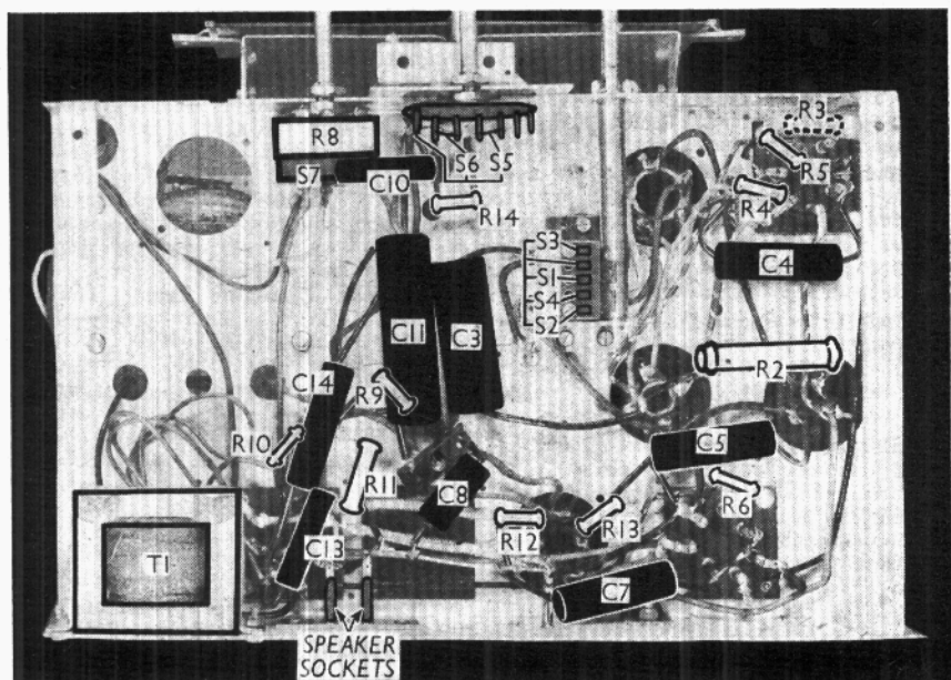
Under-chassis view. All the switches are indicated.
