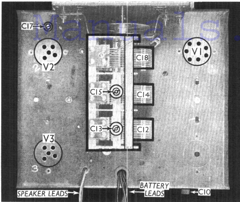
Plan view of the chassis. Note the position of C17.
