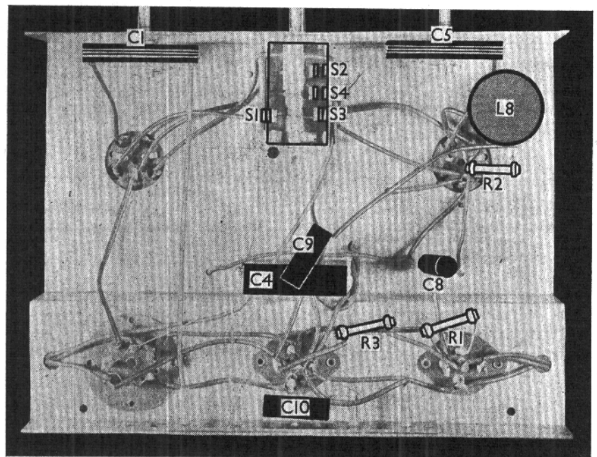
Under-chassis view. There are very few components, and even the switch unit is very simple. C 1 and C 5 are the volume-selectivity and reaction condensers respectively, while L 8 is the detector anode H.F. choke.
