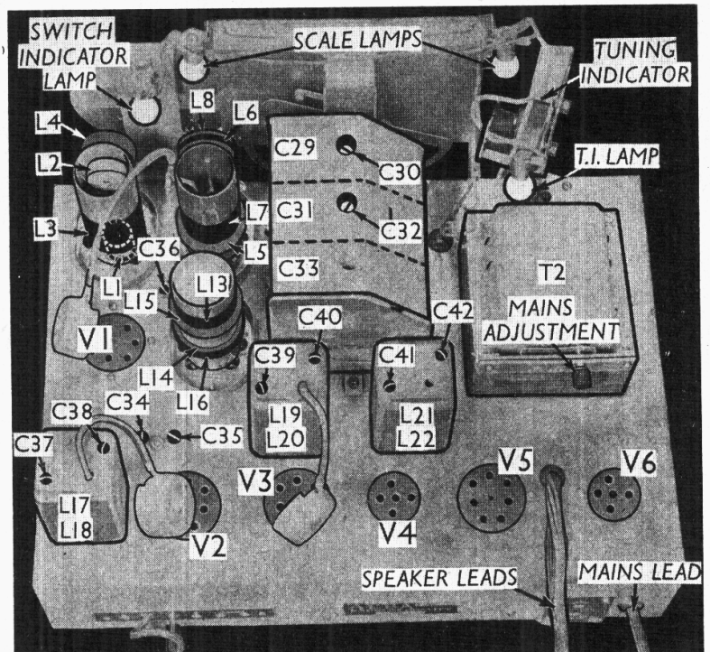
Plan view of the Alba 880 chassis. Three of the coil screens have been removed. Note that L1 is inside the main former of one unit, near the chassis. The trimmers of C33 ( C34 and C35 ) are adjusted through holes in the chassis deck, as is also C36 .
