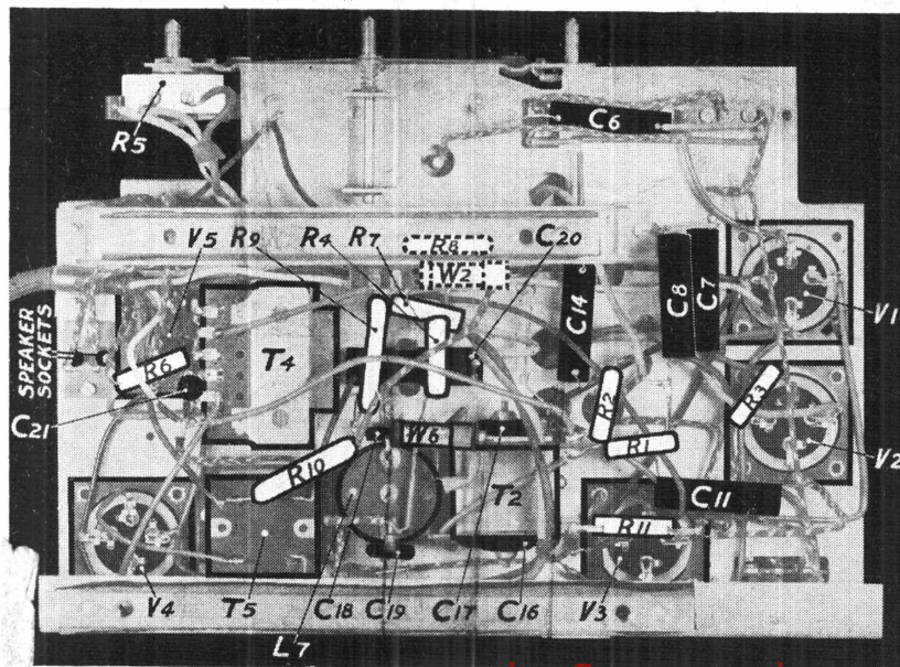
Fig. 3. Under-chassis view.
